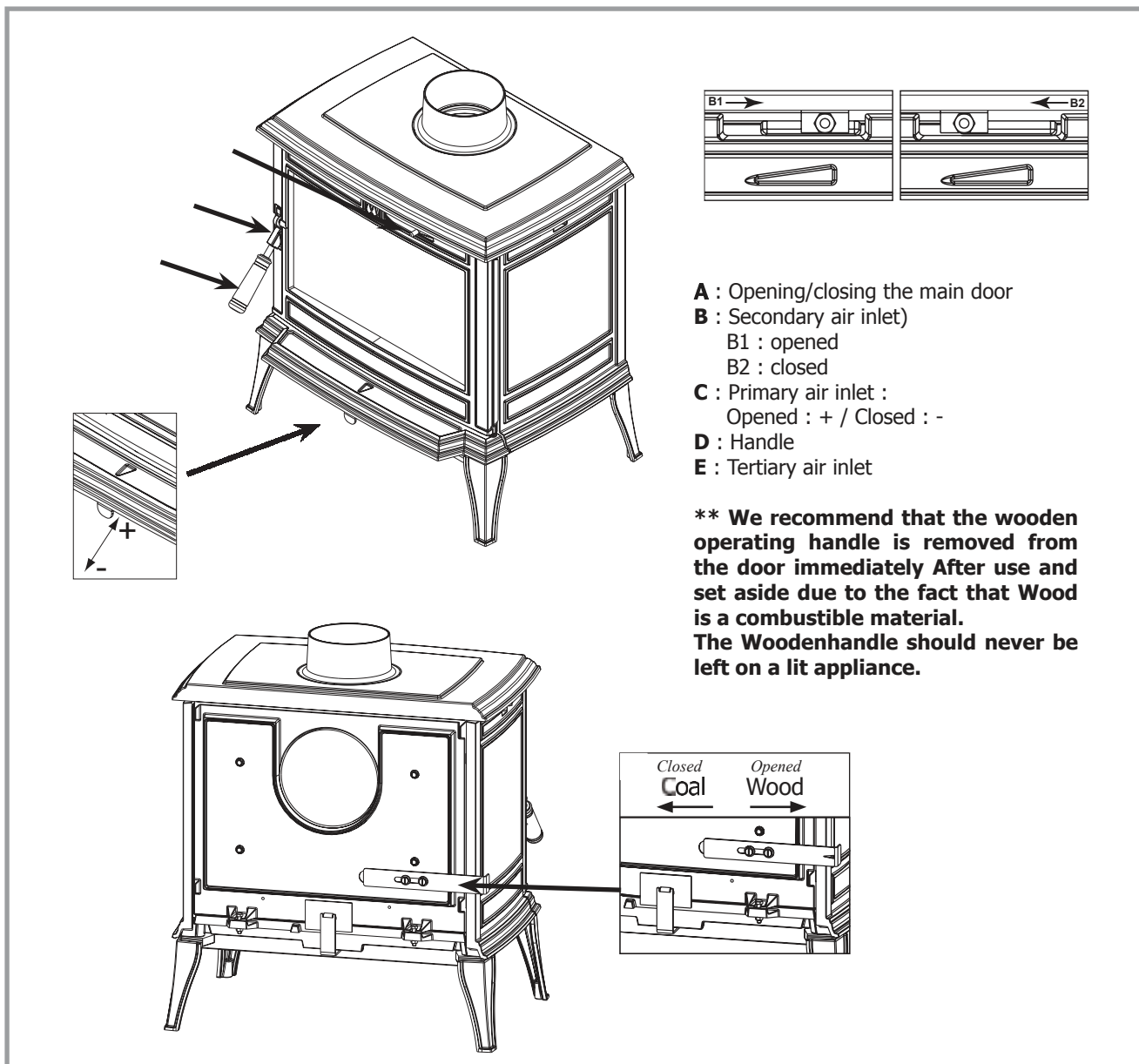
Figure 8 * Operating devices
