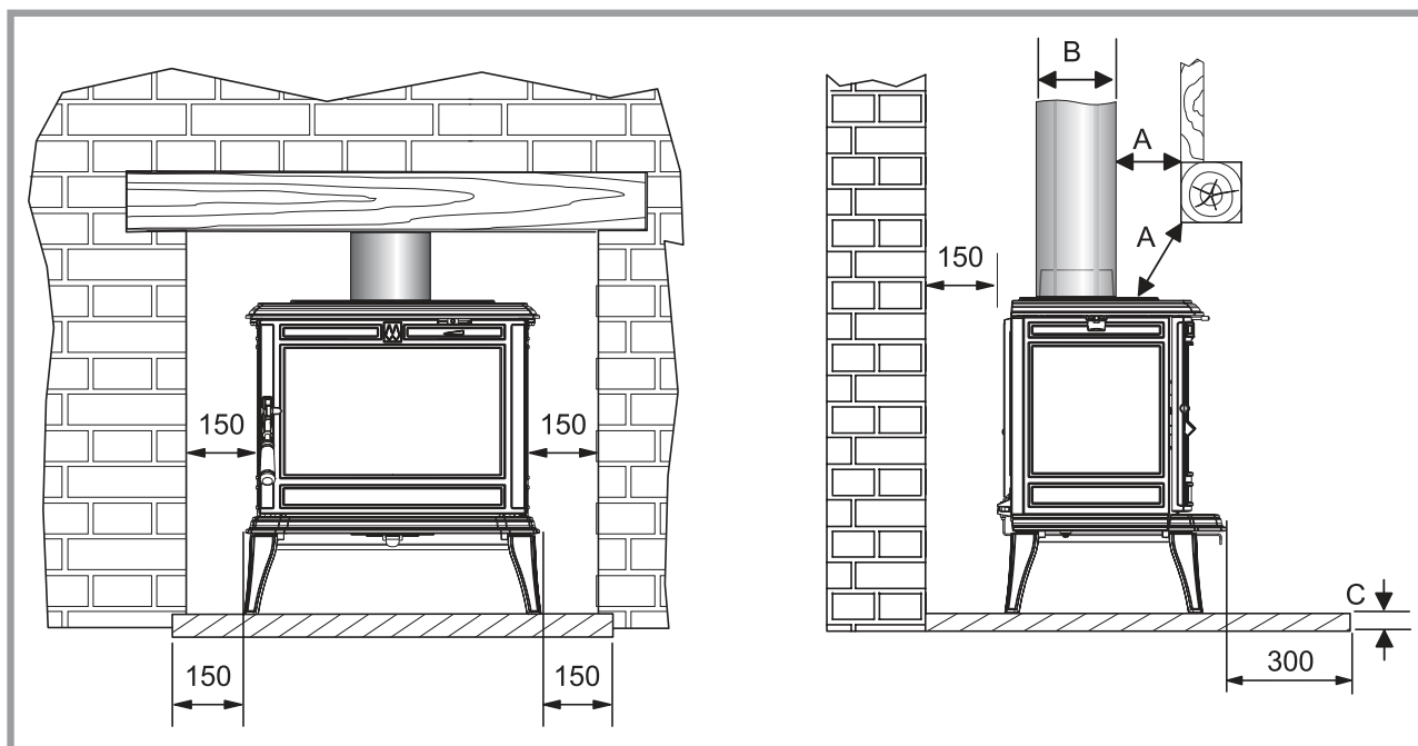
Figure 3 - Minimum clearances
